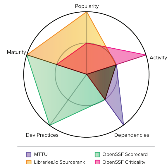
FIGURE 2.5 OPEN SOURCE QUALITY METRIC COMPARISON
